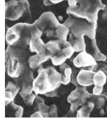
Figure 2. Sintered Tantalum
